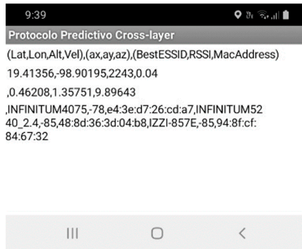
Figure 6. Screenshot smartphone.
