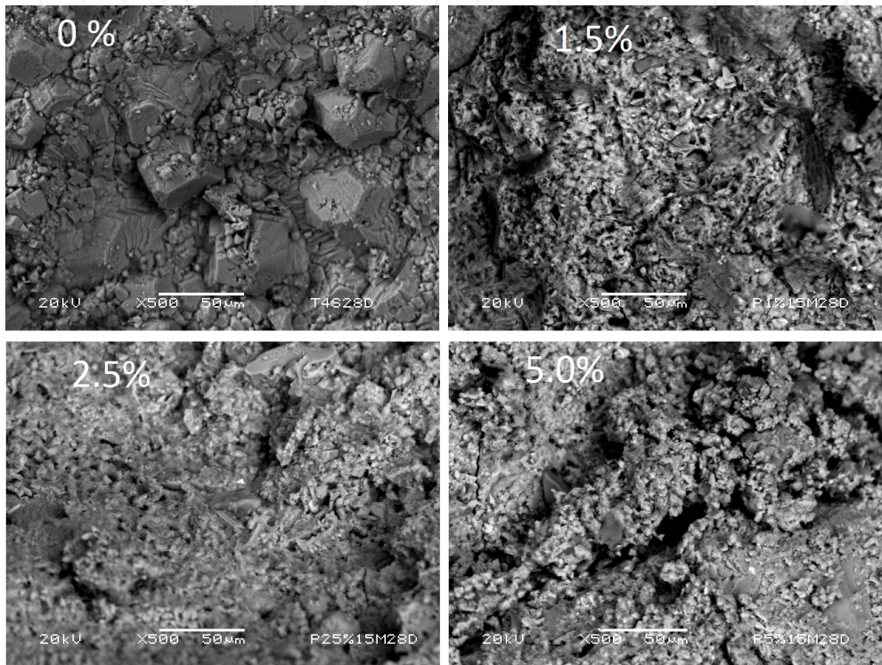
Figure 1. Concrete with different concentrations of PET particles
