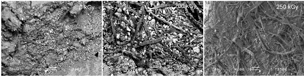
Figure 5. SEM images of gamma-irradiated concrete with tire rubber fibers
