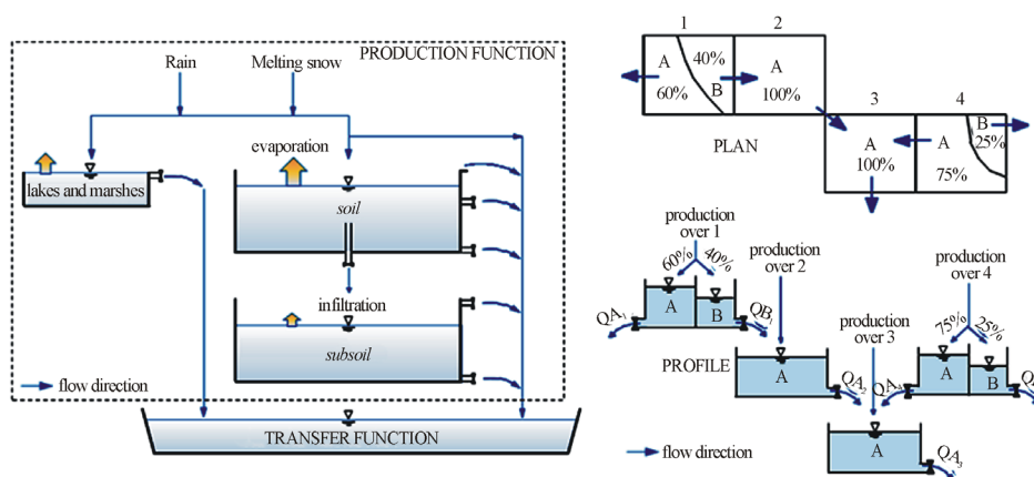
Figure 1. Production function (left) and transfer function (right) for the distributed hydrological model.
