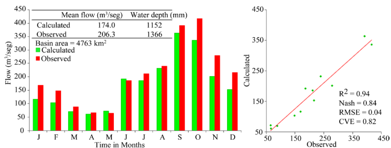
Figure 12. Calculated and observed monthly mean flows (m 3 /sec) at the Pueblo Nuevo station (30016) using the implemented CEQUEAU hydrological model, Penman-Monteith FAO 56.
