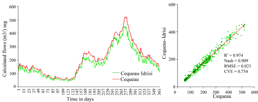
Figure 6. Comparison between inter-annual flows (mm) calculated with the CEQUEAU model and the model implemented in Idrisi.
