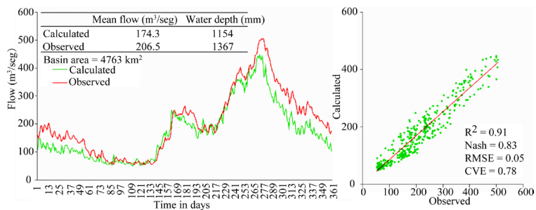
Figure 11. Calculated and observed inter-annual daily flows (m 3 /sec) at the Pueblo Nuevo station (30016) using the implemented CEQUEAU hydrological model, Penman-Monteith FAO 56.
