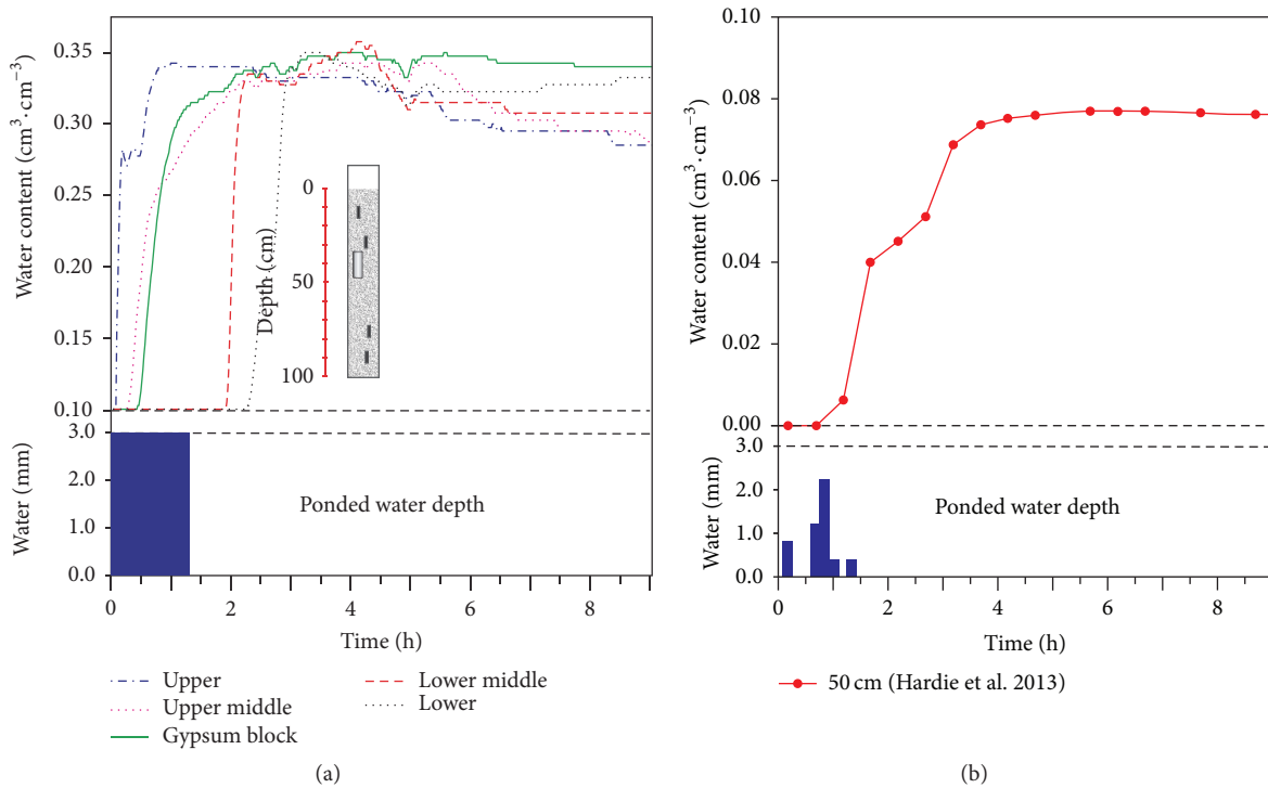
FIGURE 6: Comparison of wetting front progression versus time as derived from (a) second infiltration test of this study measured by electrical resistance sensors and (b) modified from Hardie et al. [19]. The ponded water depth at the upper boundary is also indicated.
