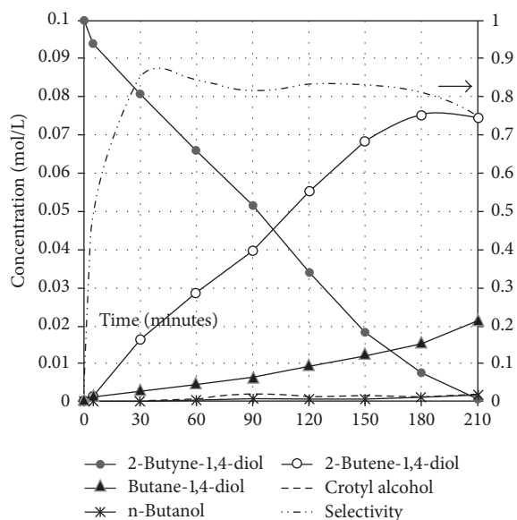
FIGURE 6: Concentration-time profile for 2-butyne-1,4-diol hydrogenation. Reaction conditions: temperature, 328 K; pressure, 6 bar; initial concentration = 0.1 mol/L; active concentration of catalyst, 0.215 mg; stirring speed, 550 rpm; total volume, 1.5 \times 10^{-4} \text{ m}^3 .
