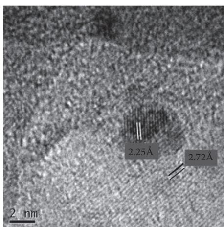
FIGURE 4: HRTEM micrograph Pt-nanobiocomposite.
