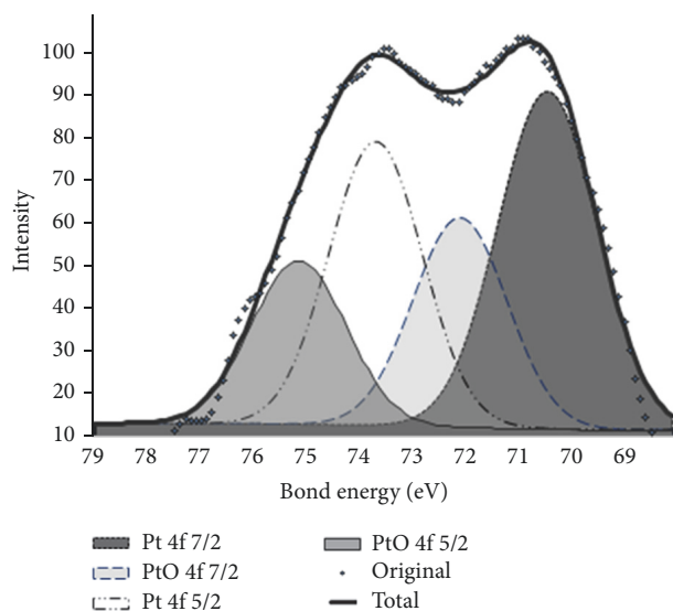
FIGURE 5: XPS spectra corresponding to the Pt 4f5/2 and 4f7/2 regions of the platinum nanoparticles supported over bovine-bone dust.
