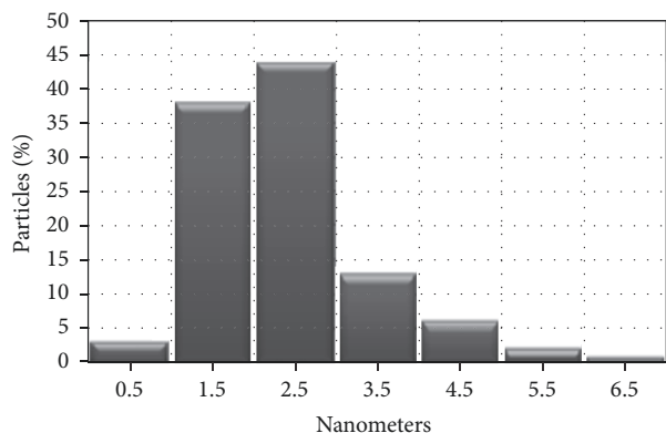
FIGURE 3: Size distribution of platinum nanoparticles.
