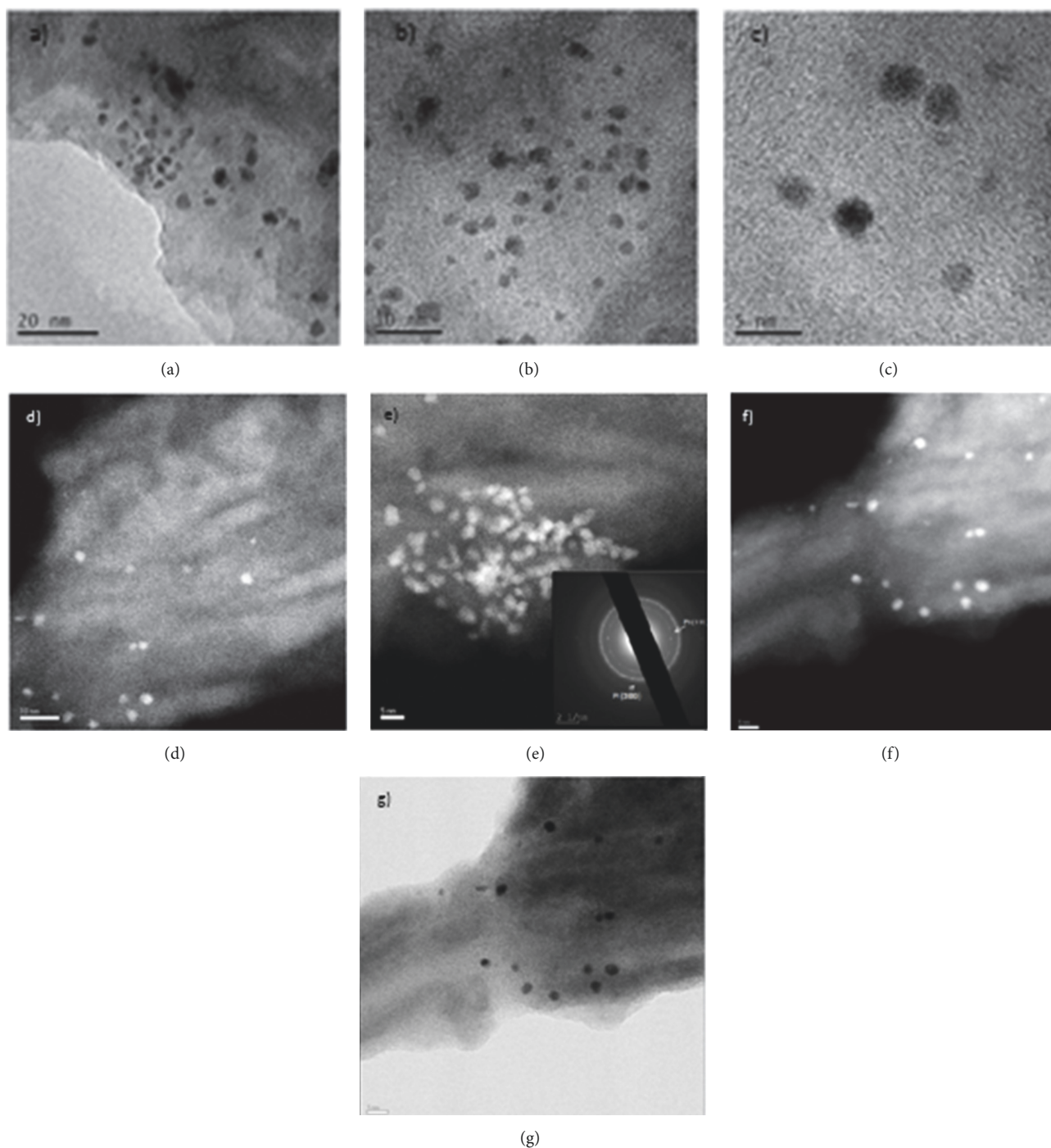
FIGURE 2: ((a), (b), (c), and (g)) BF-STEM images of Pt nanoparticles in bovine-bone powder, in different magnifications 200 kV. ((d), (e), and (f)) HAADF-STEM images of supported Pt nanoparticles on bovine-bone powder.
