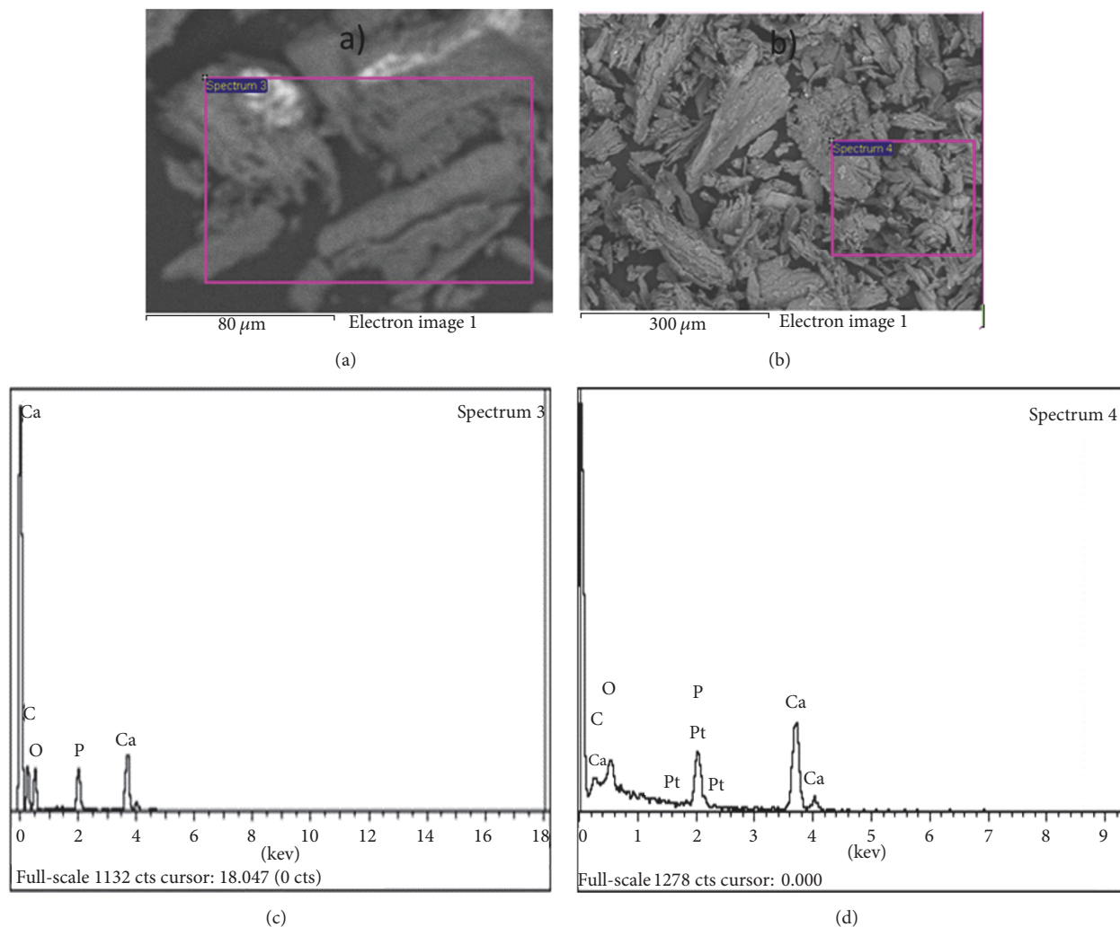
FIGURE 1: (a) SEM image of bovine-bone powder, 20 kV. (b) SEM image of bovine-bone powder after the synthesis of nanoparticles of platinum, 20 kV. (c) EDS spectrum: the analyzed area is indicated by the pink square. ((a) and (d)) EDS spectrum: the analyzed area is indicated by the pink square in (b).
