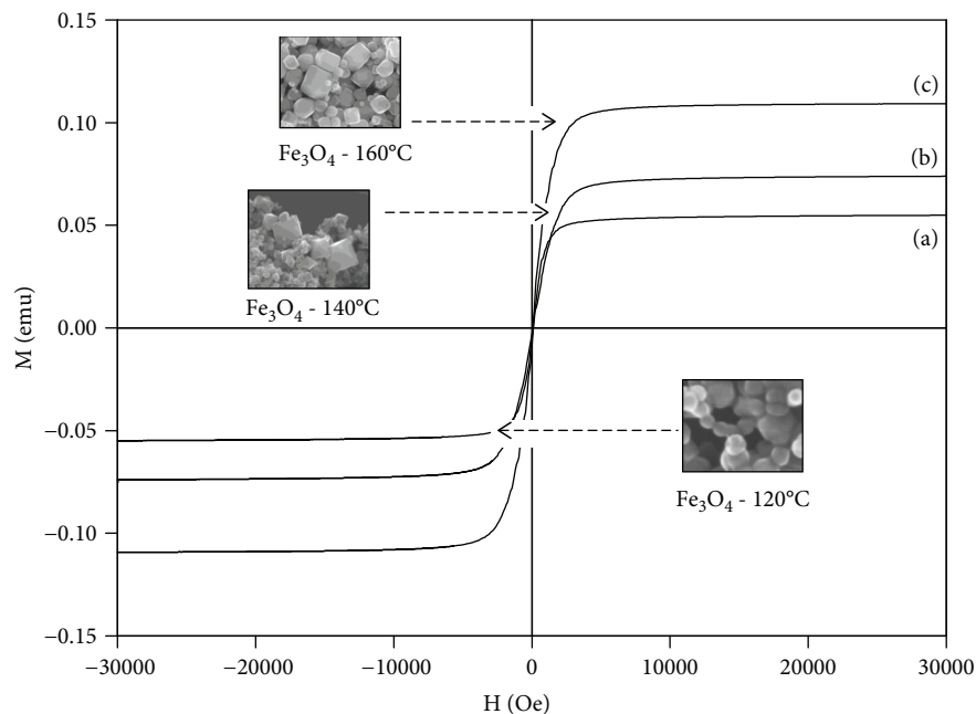
FIGURE 8: Magnetization curves at room temperature of \text{Fe}_3\text{O}_4 nanoparticles. (a) 120°C. (b) 140°C. (c) 160°C.
