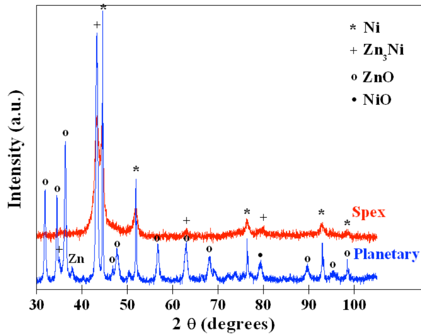
Figure 2. XRD comparative graph of the milled and sintered samples, showing the found phases.
